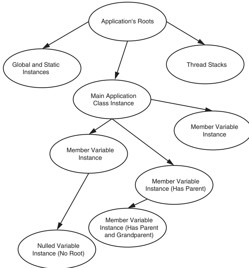
Figure 2.3 Root reference tree
