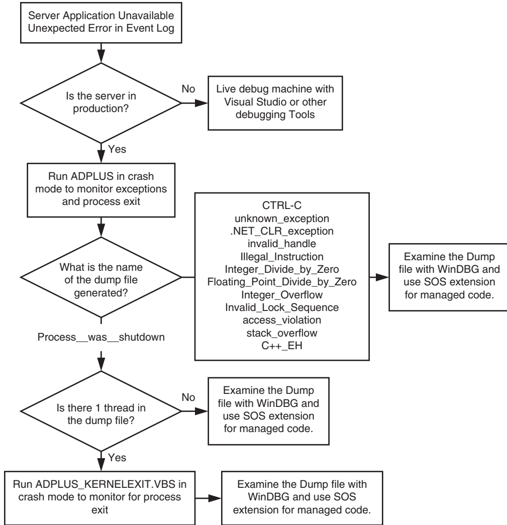
Figure 4.1 Thought Process Flowchart
