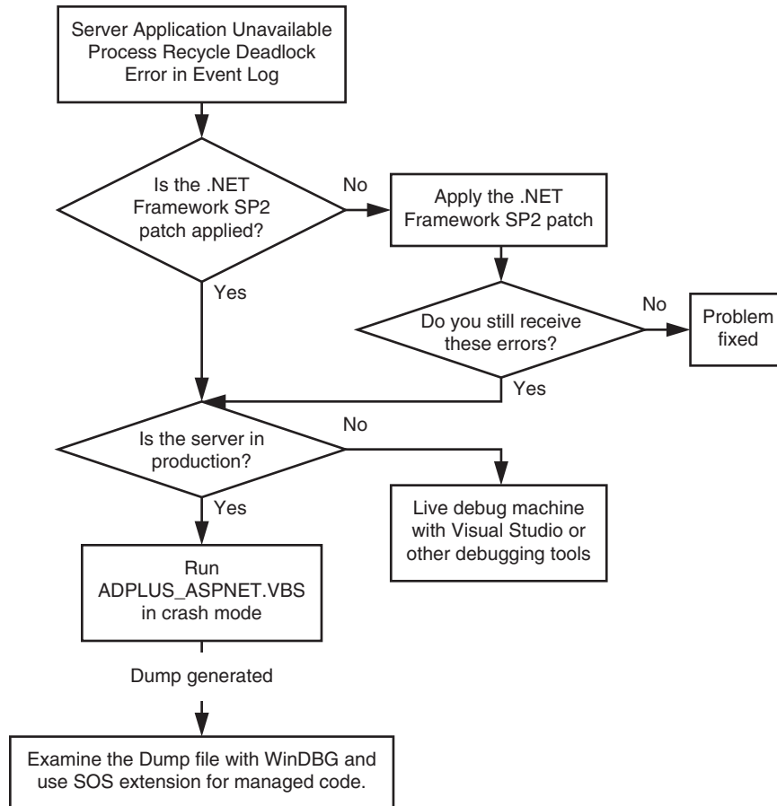
Figure 3.2 Thought flowchart
