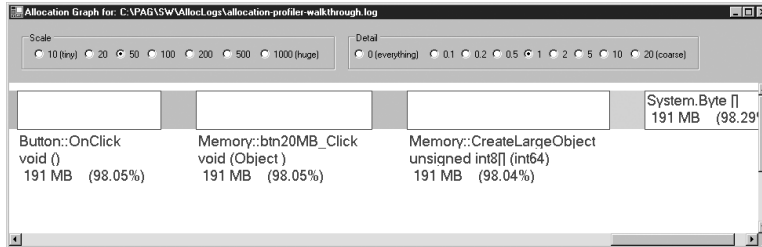
Figure 2.15 Allocation graph
