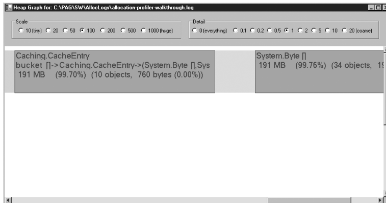
Figure 2.16 Heap graph
